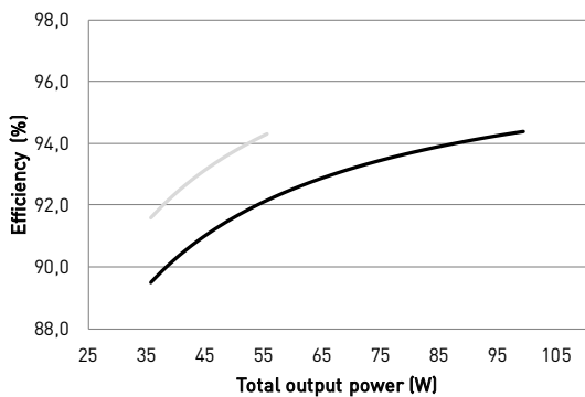
Typical efficiency
