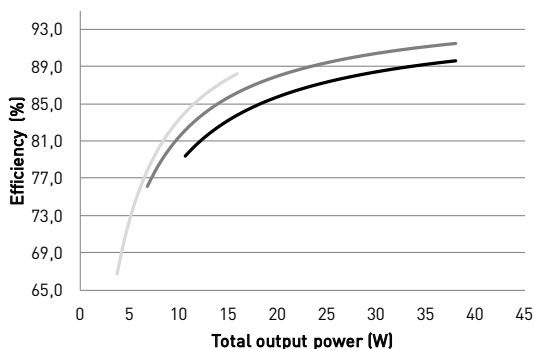
Typical efficiency
