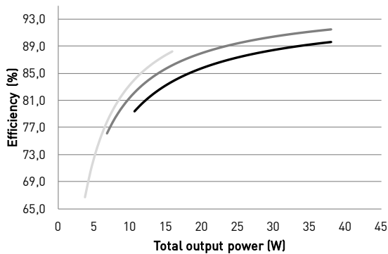
Typical efficiency
