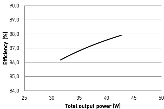
Typical efficiency
