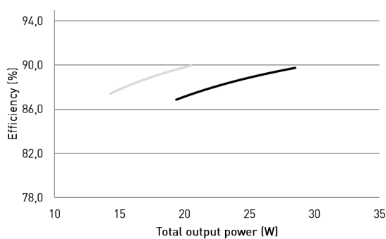
Typical efficiency
