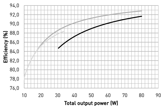
Typical efficiency
