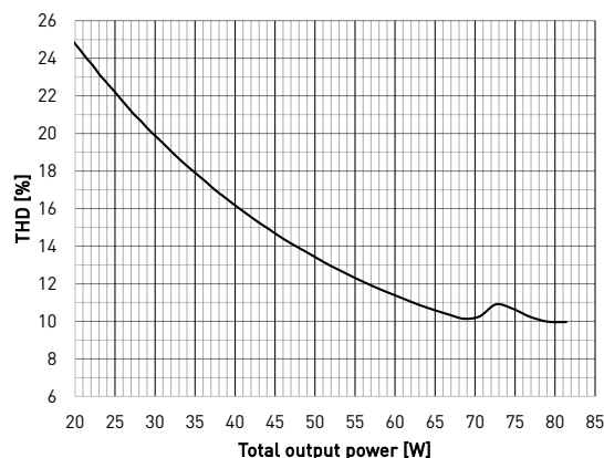
Current THD
