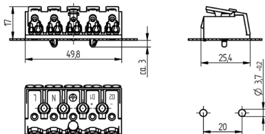
5 - pole LOOPing connector
